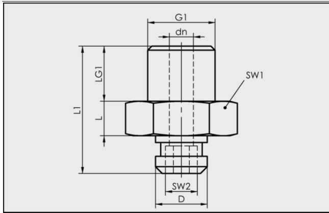
Design data SA-NIP N022 G1/8-AG DN350
