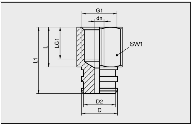
Design data SA-NIP N023 G1/4-IG DN350
