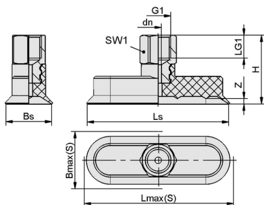
Design data SGON 15x5 NBR-55 M5-IG
