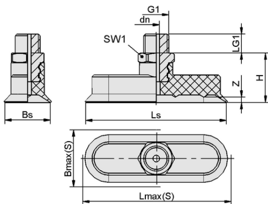
Design data SGON 30x10 NBR-55 G1/8-AG
