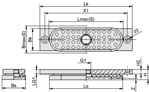
Design data SPLO 60x20 NBR-55 G1/8-IG
