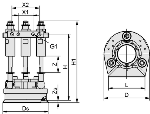
Design data DBD 100x145 36 M42
