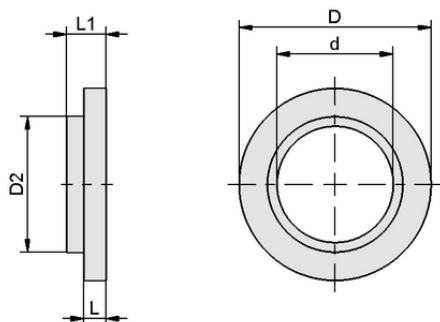
Design data SCHE 38-18.5x5 ST VZ
