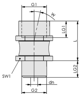
Design data FLK G1/2-IG G1/2-AG
