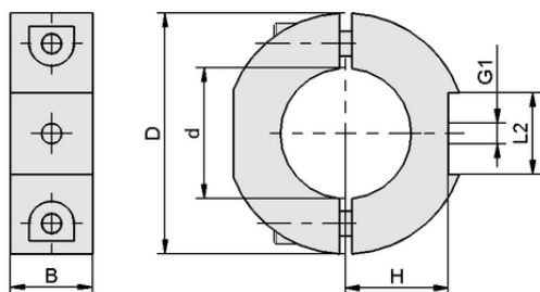
Design data HTR-STC D32 UNI
