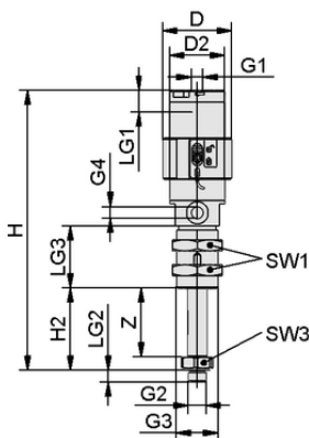
Design data FST-LOCK-HD G1/4-AG 50 NC VG SFP
