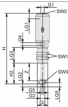
Design data FST-LOCK-HD G1/4-AG 100 NC AB
