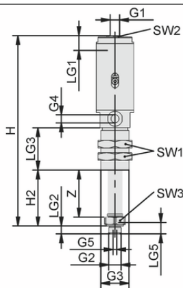
Design data FST-LOCK-HD G1/4-AG 50 NC AB
