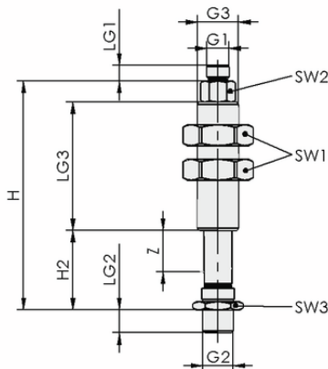
Design data FSTI G1/4-AG G1/8-AG 25 VG
