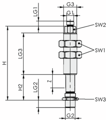
Design data FSTI G3/8-AG G1/8-AG 10 VG
