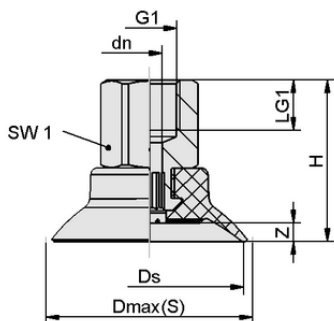
Design data SUF 30 HT1-60 NPT1/8-IG
