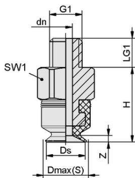
Design data PFYN 3.5 NBR-ESD-55 M3-AG
