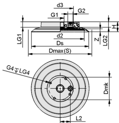
Design data SGF-HS 150 EPDM-55 G1/2-IG
