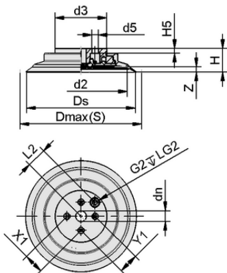
Design data SGF-HS 150 HT1-60 FM1
