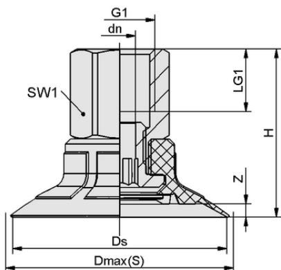
Design data SPF 60 ED-65 G1/4-IG
