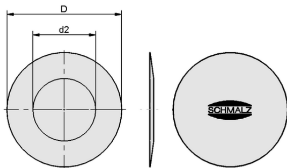
Design data PC 300
