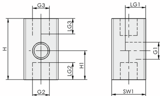
Design data ANW M5-IG M3-IG
