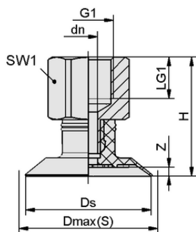
Design data SGPN 40 HT1-60 G1/4-IG
