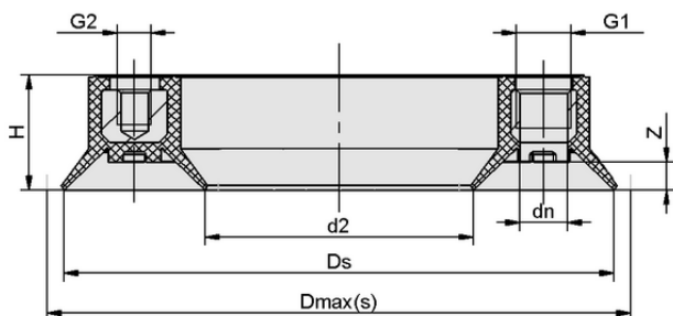
Design data SR-DBD 100 NBR-60
