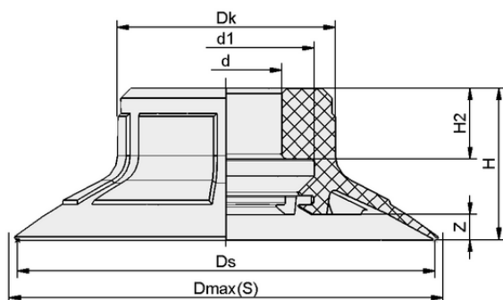
Design data SPF 40 ED-65 SC050
