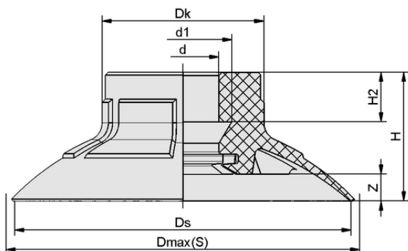
Design data SPF 25 ED-65 SC040
