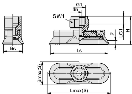
Design data SAOG-S 95x40 NBR-60 G3/8-IG
