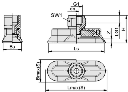
Design data SAOG-S 60x20 NBR-60 G1/4-IG
