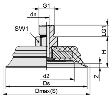
Design data SHFN 85 NK-45 G1/4-AG E
