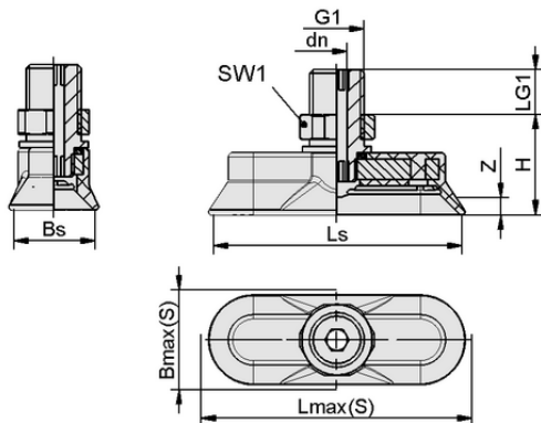
Design data SAOG-S 80x30 NBR-60 G1/4-AG
