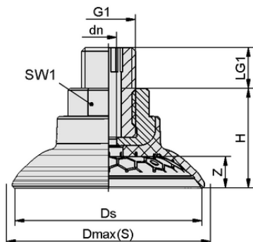
Design data SAG 80 NBR-60 G1/4-AG
