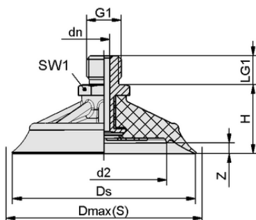
Design data SHFN 85 NK-45 G1/4-AG TV
