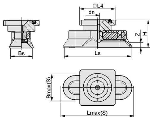
Design data SAOG 60x20 NBR-45 RA
