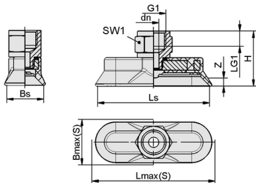
Design data SAOG 60x20 NBR-45 G3/8-IG
