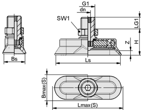
Design data SAOG 60x20 NBR-45 G1/4-AG
