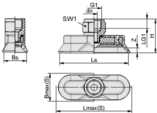
Design data SAOG 60x20 NBR-45 G1/4-IG
