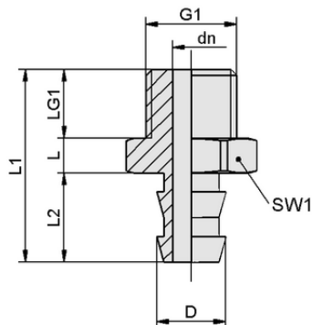
Design data SA-NIP N035 G1/8-AG DN500
