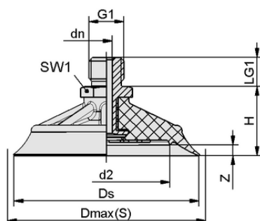
Design data SHFN 50 NK-45 G1/4-AG MOS-TV
