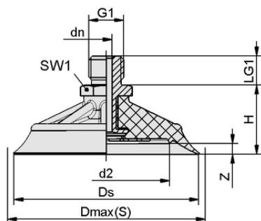
Design data SHFN 50 NK-45 G1/4-AG TV
