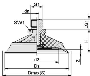
Design data SHFN 70 NK-45 G1/4-AG MOS-TV
