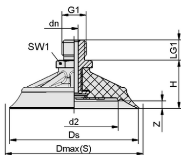
Design data SHFN 70 NK-45 G1/4-AG TV
