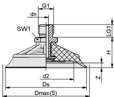
Design data SHFN 50 NK-45 G1/4-AG
