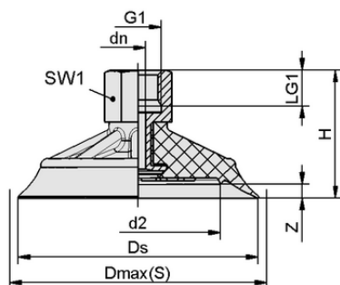
Design data SHFN 70 NK-45 G1/4-IG
