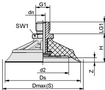
Design data SHFN 70 NK-45 G1/4-AG
