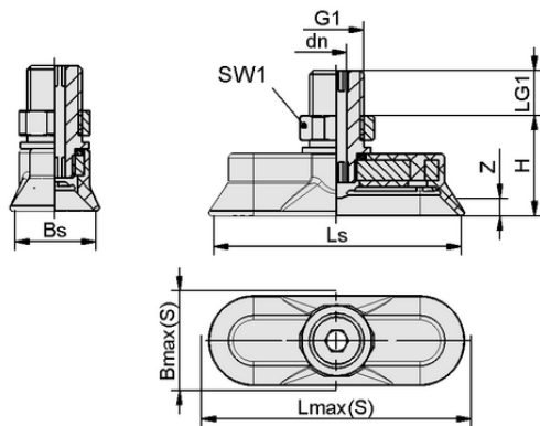
Design data SAOG 80x30 NBR-45 G3/8-AG
