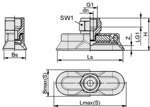
Design data SAOG 80x30 NBR-45 G3/8-IG
