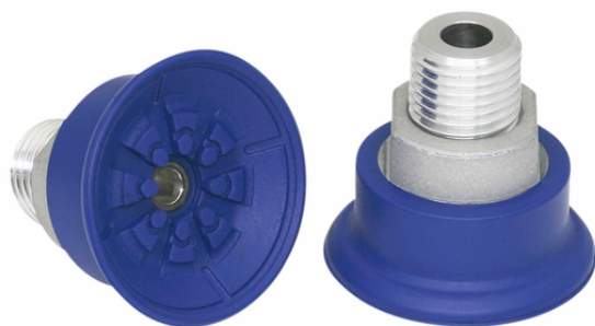
SAF 30 NBR-60 G3/8-AG
