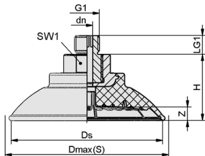
Design data SAF 50 NBR-60 M10-AG
