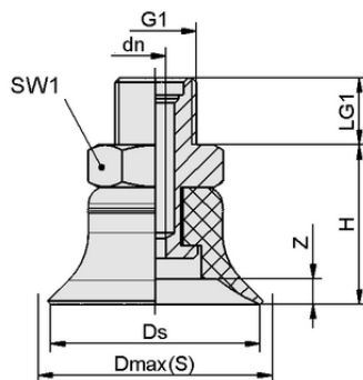
Design data PFYN 40 NBR-CO-55 G1/8-AG
