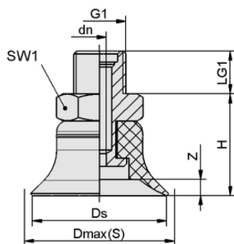
Design data PFYN 30 NBR-CO-55 G1/8-AG
