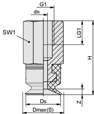
Design data PFYN 10 SI-CO-55 G1/8-IG
